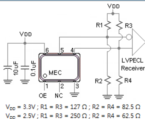
LVPECL Test Circuit
