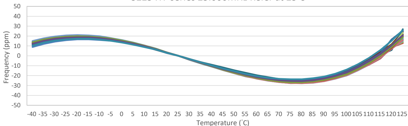
3225 HY-series 25.000MHz Refer at 25°C
